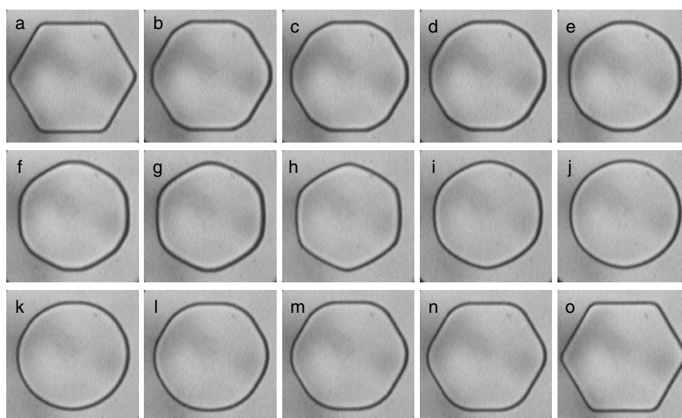
Figure 1. Sequence of melting and growth shapes of an ice crystal in pure water observed in a high pressure anvil cell. The pressure is held at 2000 bar and hence the bulk coexistence temperature is -22^{\circ}\text{C} . The axis of observation is parallel to the crystallographic c -axis, and hence each corner is collinear with one of the a -axes and the six prism facets are clearly visible. Starting from the growing shape, which is a hexagonally faceted ice crystal (a), the ice crystal undergoes a series of changes upon slight warming ((b)–(g)) in which it develops a hexagonal shape (g) that is rotated compared to the initial shape (a). On reversing the process by slightly cooling below the melting point, this ice crystal grows again ((i)–(n)) and develops a faceted hexagonal shape (o) that is identical to the starting shape (a) and rotated compared to the melting shape (h). The sequence, which takes 700 s, was taken from [1]. Courtesy of the authors and with permission from APS.
