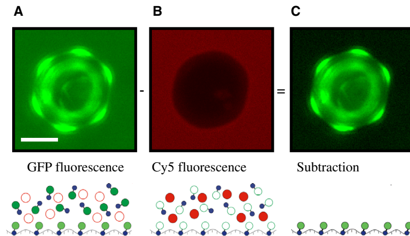
Figure 4. Image analysis for selective detection of ice-bound sbwAFP-GFP . Ice crystals were produced in a solution containing sbwAFP-GFP and a free dye (Cyanine 5-dUTP or Cy5) and imaged with 488 and 633 nm illumination lines through two separate fluorescence filters: a Cy5 filter, and a GFP filter. (A) GFP fluorescence alone. White scale bar represents 7 \mu\text{m} . (B) Cy5 fluorescence alone. (C) Subtraction of the Cy5 image from the GFP image. The lower parts of panels (A)–(C) illustrate the molecules present: GFP, large (green) circles in the dumbbells; Cyanine 5, stand alone (red) circles. Filled circles represent molecules detected by fluorescence with a particular optical filter and empty circles denote molecules that are not detected; sbwAFP domains are the small (blue) circles in the dumbbells. The lower parts of the panels were adapted from figure 3(D) in [26] with permission from Biophysical Journal.
