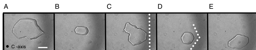
Figure 2. Growth–melt asymmetry of an ice crystal in a solution containing 10\ \mu\text{M} spruce budworm ice binding protein: bright field measurements. (A)–(E) Snapshots from a movie (supplementary materials Movie S1 available at stacks.iop.org/JPhysCM/19/412101 ) showing the growth and melting of the ice crystal. At the sbwAFP-GFP concentration used ( 10\ \mu\text{M} ), the thermal hysteresis is 0.07\ ^\circ\text{C} . The temperature was alternated between 0.02\ ^\circ\text{C} above the melting point of the solution and 0.02\ ^\circ\text{C} below the temperature of rapid crystallization, forcing the ice crystal to melt ((B), (D)) or grow ((C), (E)) in a controlled manner. The images clearly show a 30^\circ shift between the planes of growth and melting of the ice crystal, which causes the ice facets such as the one near the dotted vertical line in (C) to form into corners such as the one near the dotted corner in (D). Scale bar in (A) represents 30\ \mu\text{m} .
