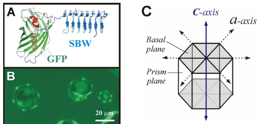
Figure 3. sbwAFP linked to GFP : fluorescence microscopy. (A) Ribbon diagram of the spruce budworm ice binding protein ( sbwAFP ) linked through its N-terminus to the C-terminus of the green fluorescent protein ( GFP ). (B) Ice crystals decorated with sbwAFP - GFP . The image was taken through a confocal microscope equipped with a GFP fluorescence filter. (C) Diagram of the basal and prism planes of an ice crystal.
