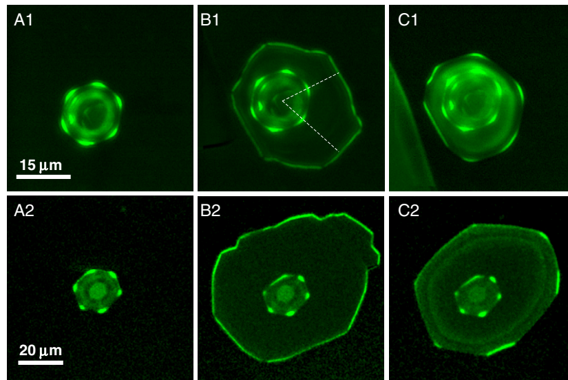
Figure 5. Growth–melt asymmetry in ice crystals in sbwAFP-GFP solution. Series 1 and 2, represent the location of the sbwAFP-GFPs on the ice crystals in an sbwAFP-GFP solution. The images are subtraction images as explained in figure 4. (A) Initial melting shapes. (B) Growing shapes. During subsequent growth the sbwAFP-GFPs are overgrown by the ice, and additional sbwAFP molecules from solution attach to the prism facets that emerge from the corners of the melt shape 30^\circ from the planes therein. (C) Partial melting. The crystal appears to have rotated again, with facets becoming corners, and the sbwAFP-GFPs are attached to the same directions as on the original melt shape, accumulating on the centers of the shrinking facets of a hexagonal ice crystal at locations that eventually become corners. A movie of experiment 2 in figure 5 (supplementary materials Movie S2 available at stacks.iop.org/JPhysCM/19/412101 ) shows the process of growth and melt.
